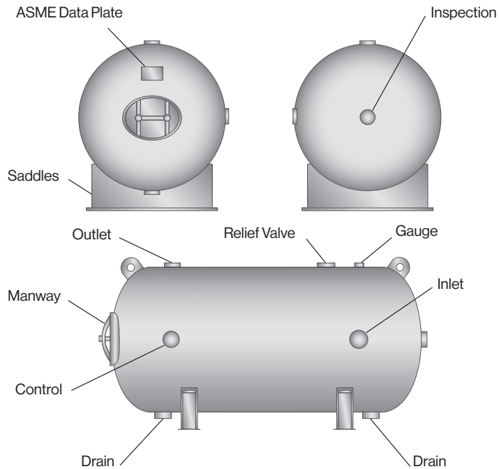
Horizontal Air Receiver
