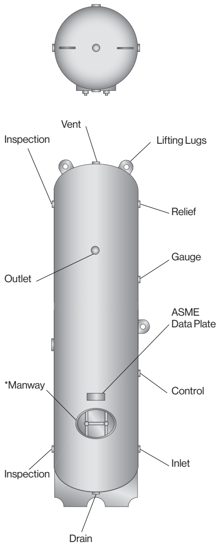
Vertical Air Receiver
