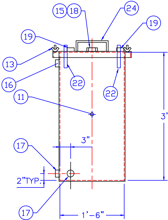
END VIEW
