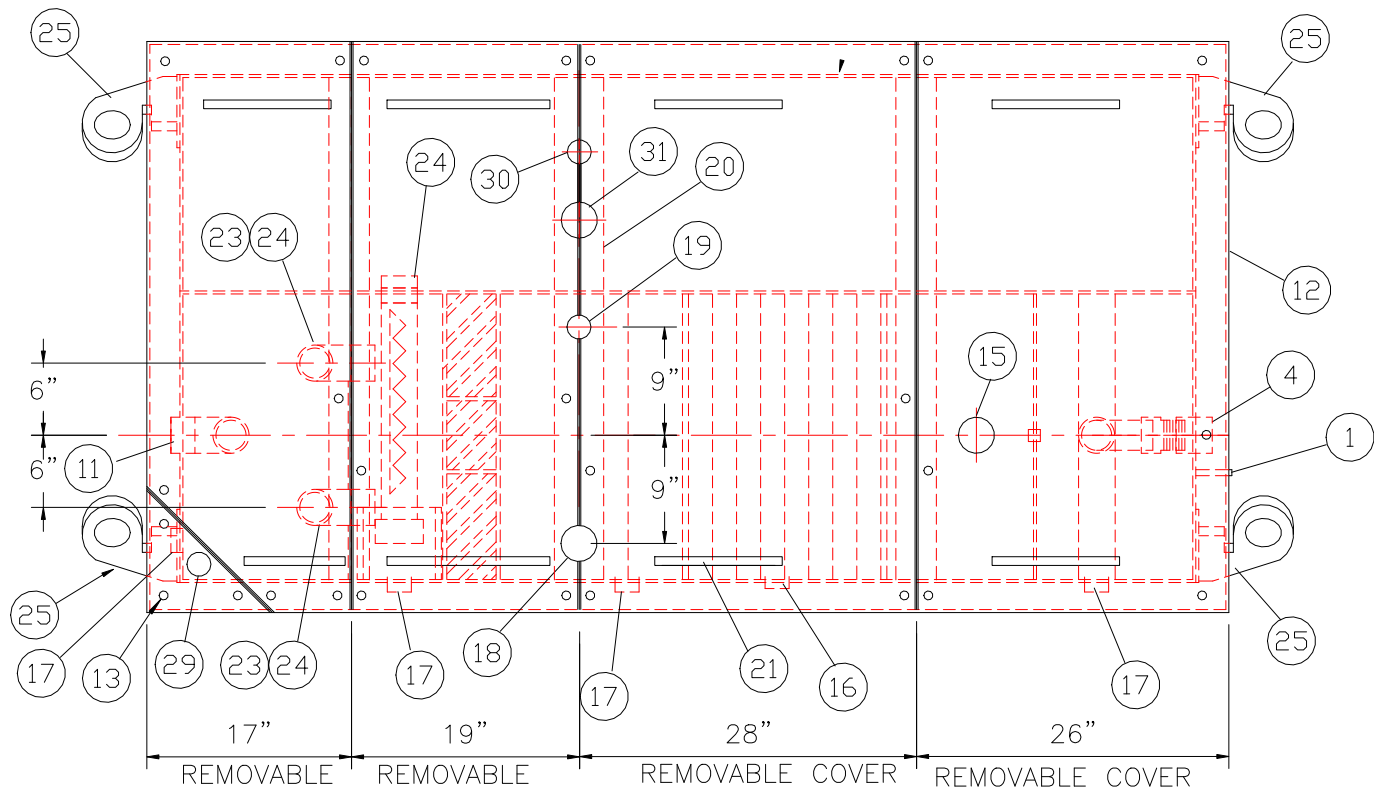
PLAN
