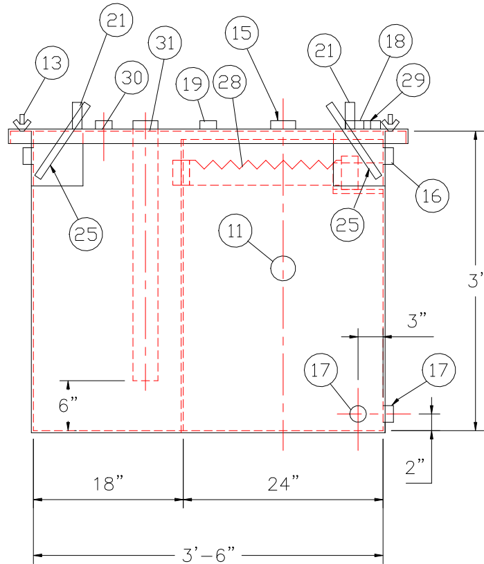
END VIEW
