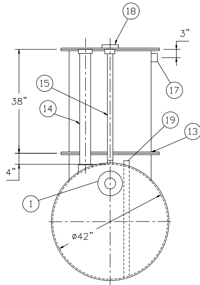
END VIEW
