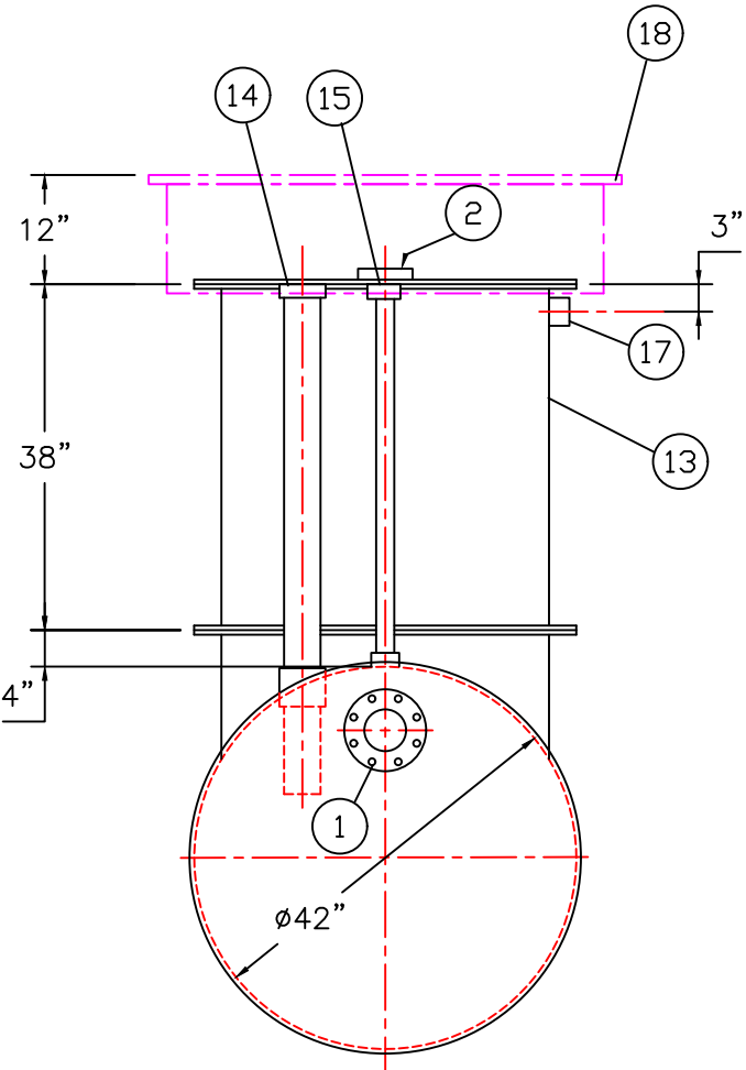
END VIEW
