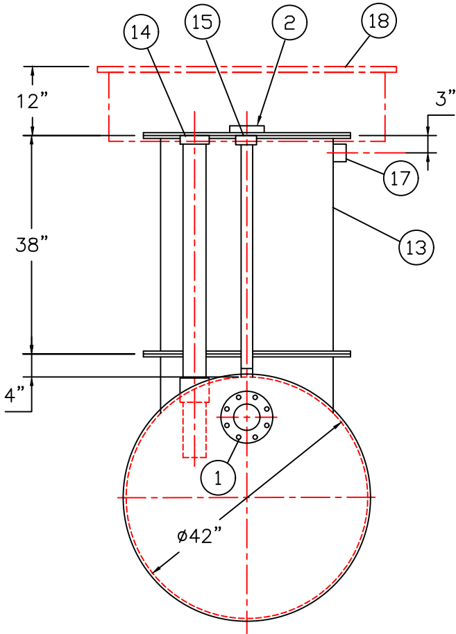
END VIEW
