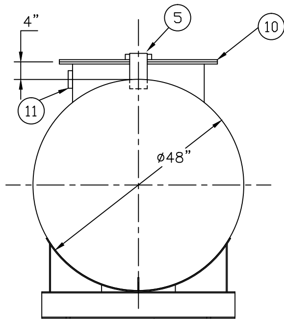
(2) 48"ø x 6" HIGH SADDLES SHIP LOOSE WITH TANK
