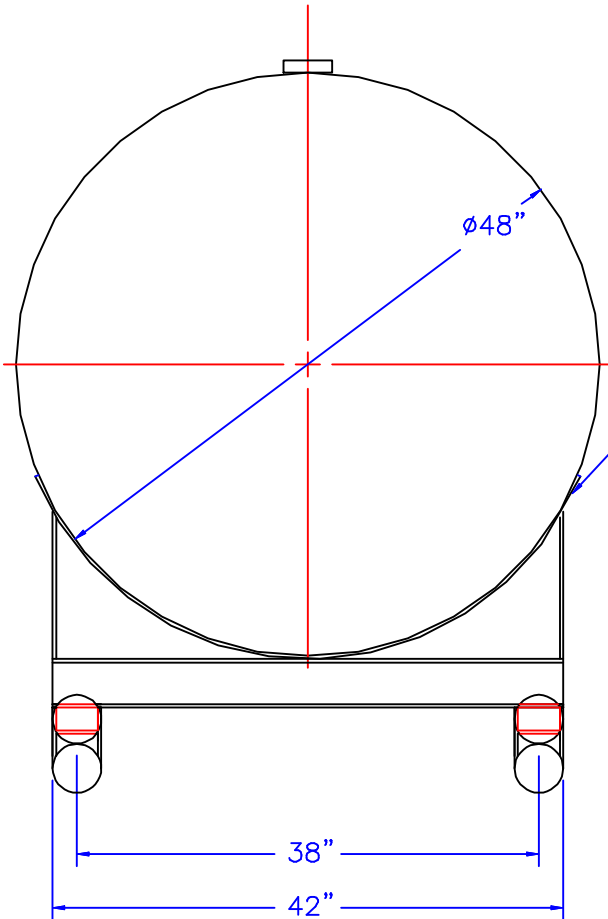
END VIEW
