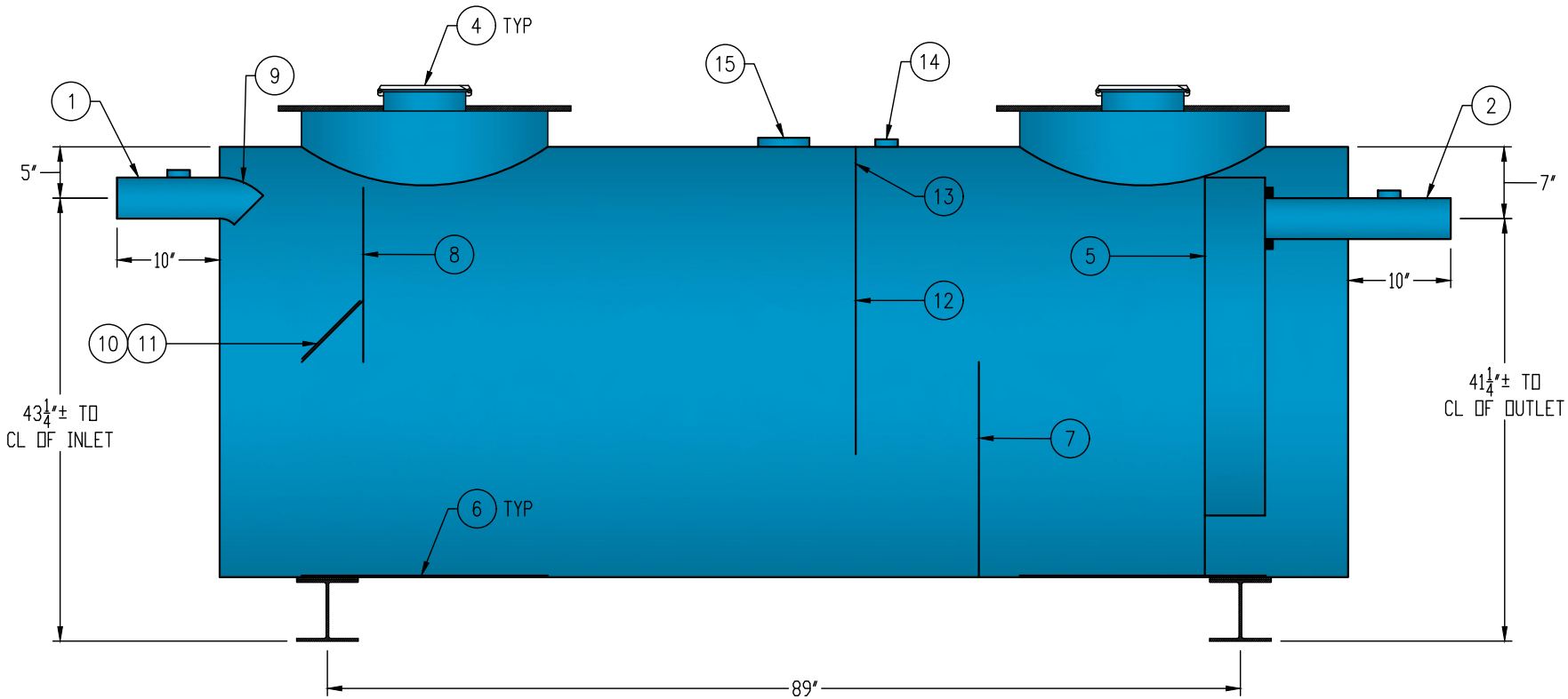
SECTION VIEW
