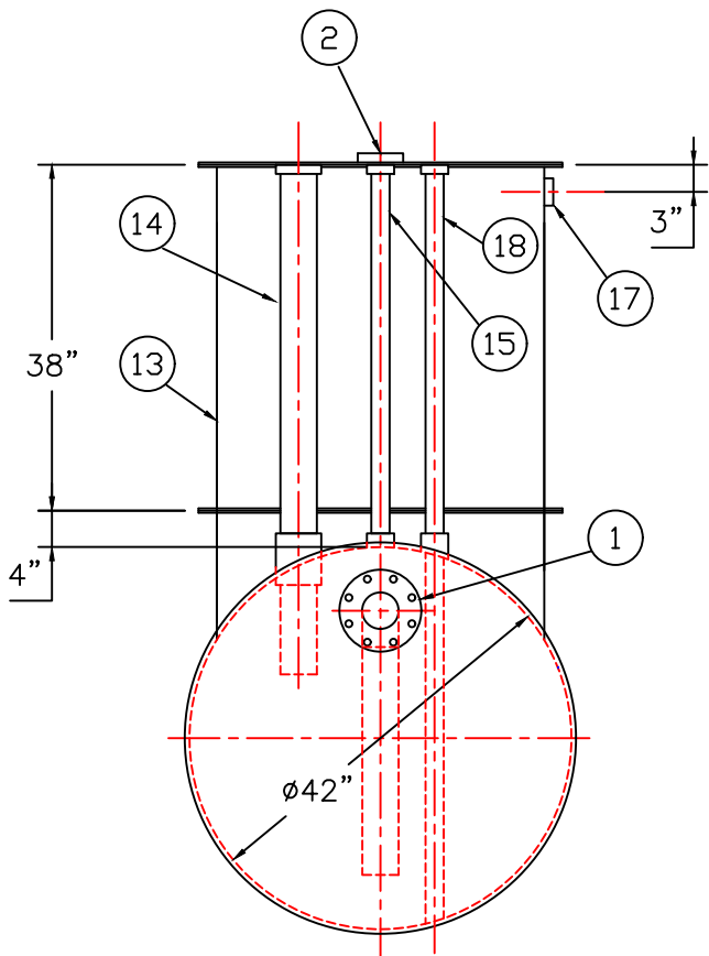
END VIEW
