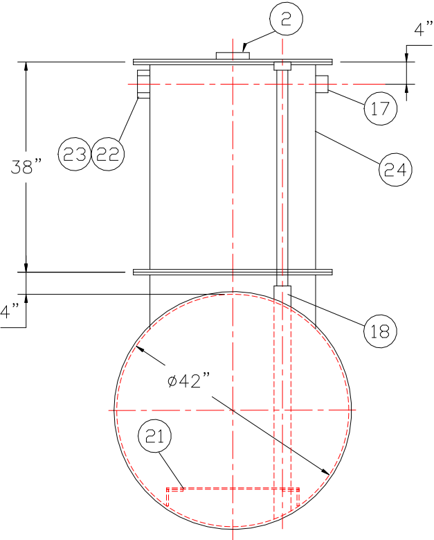
END VIEW
