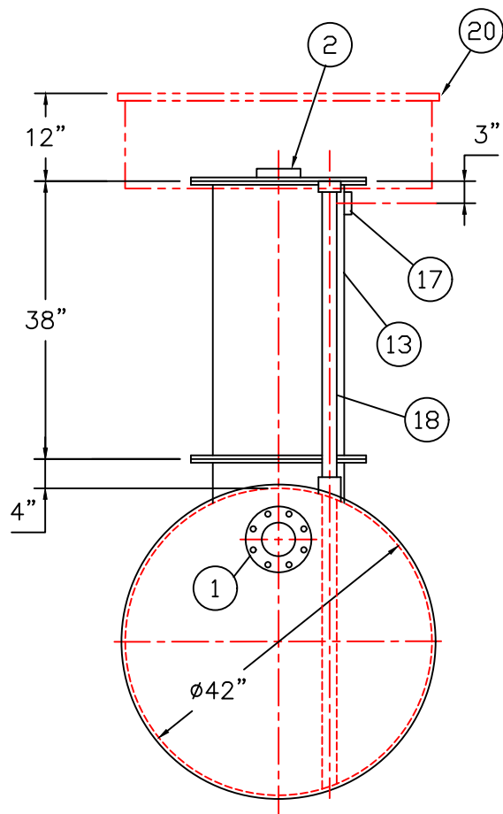
END VIEW
