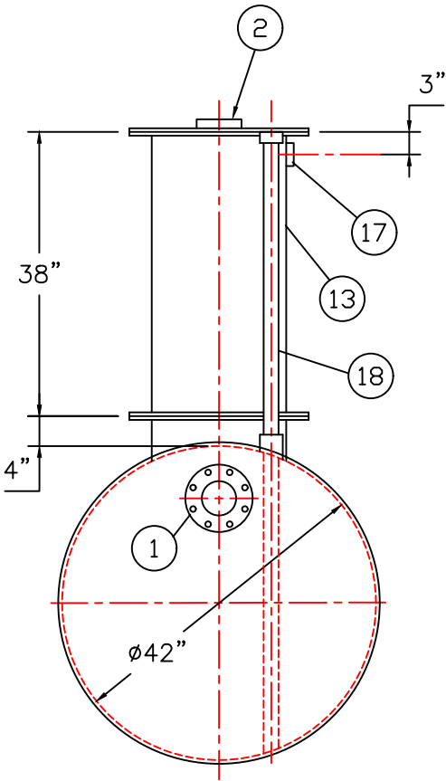
END VIEW
