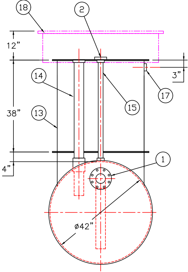
END VIEW
