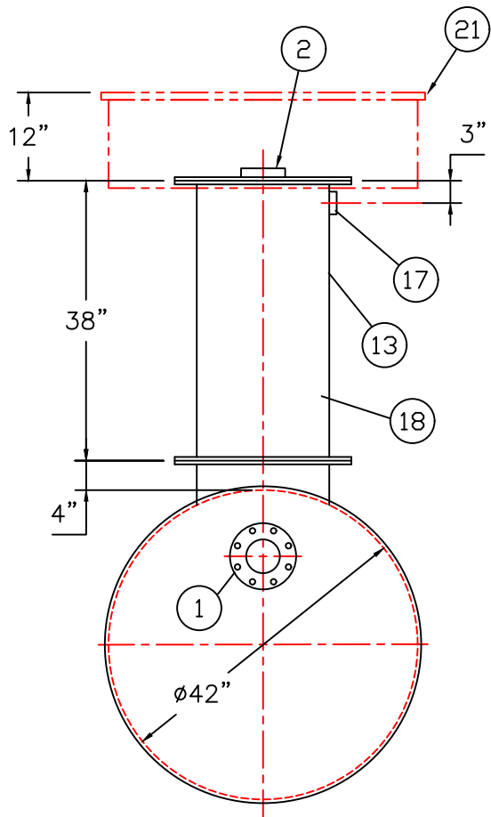
END VIEW
