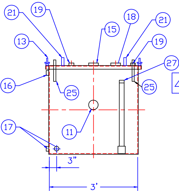
END VIEW
