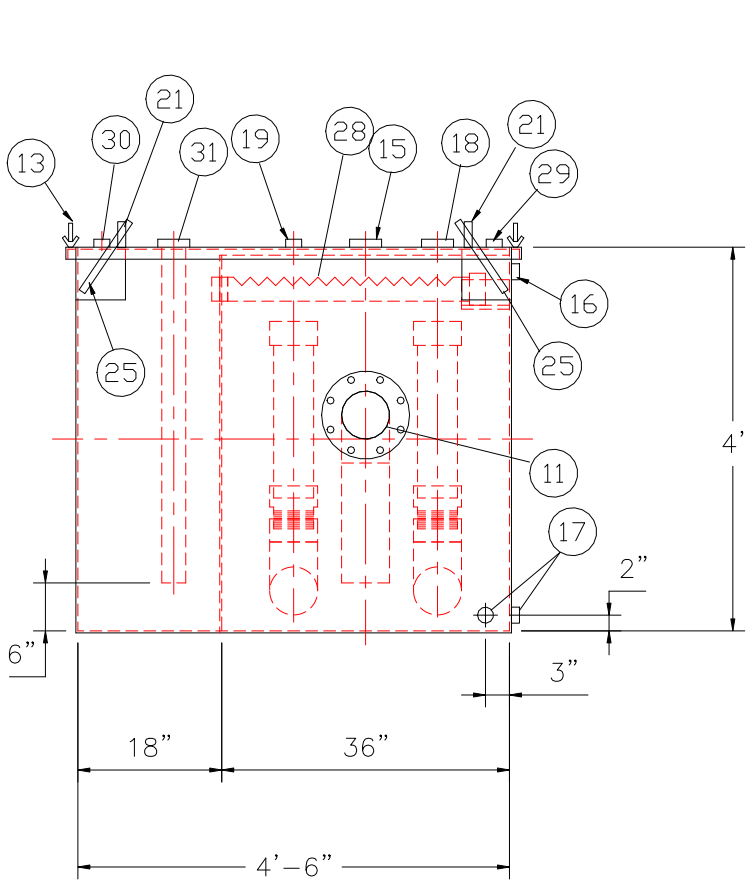
END VIEW
