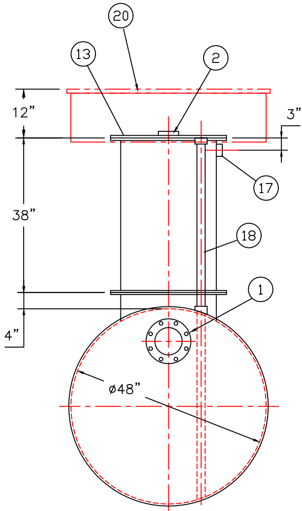
END VIEW
