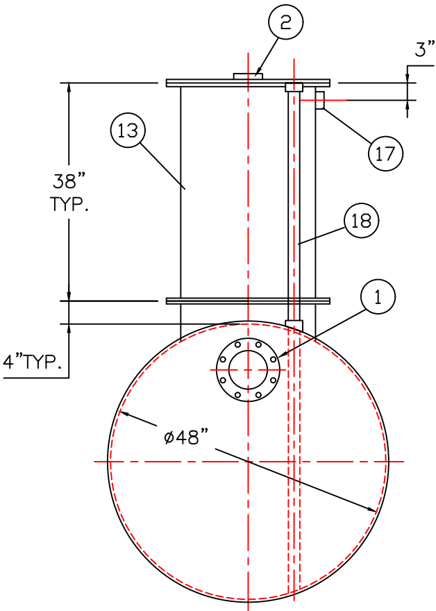
END VIEW
