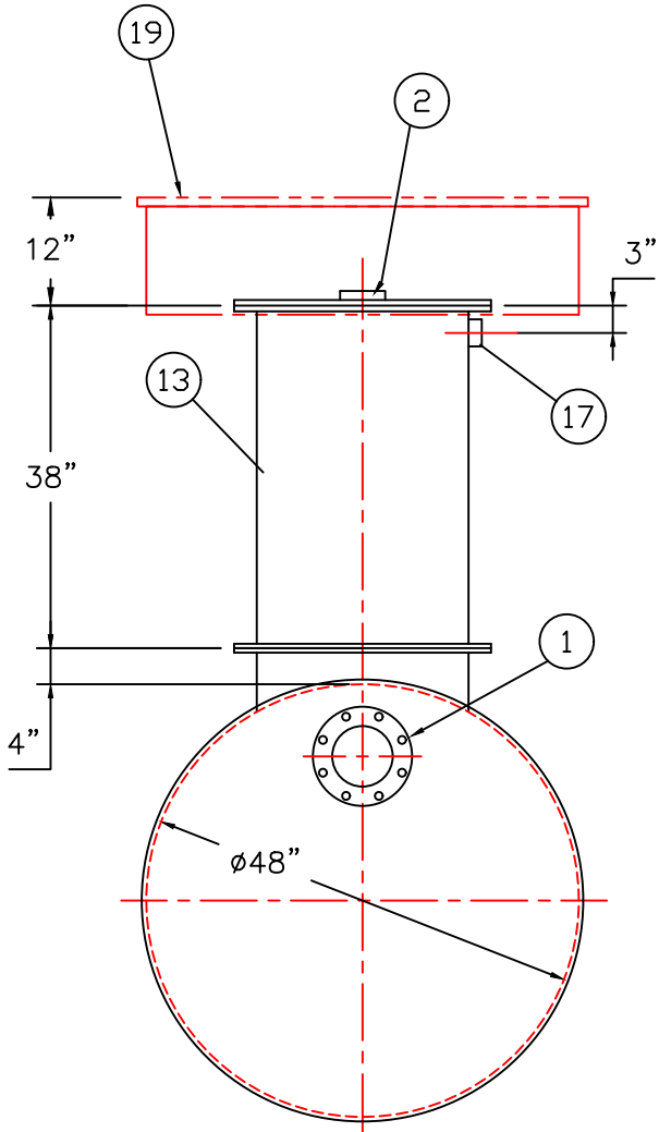
END VIEW
