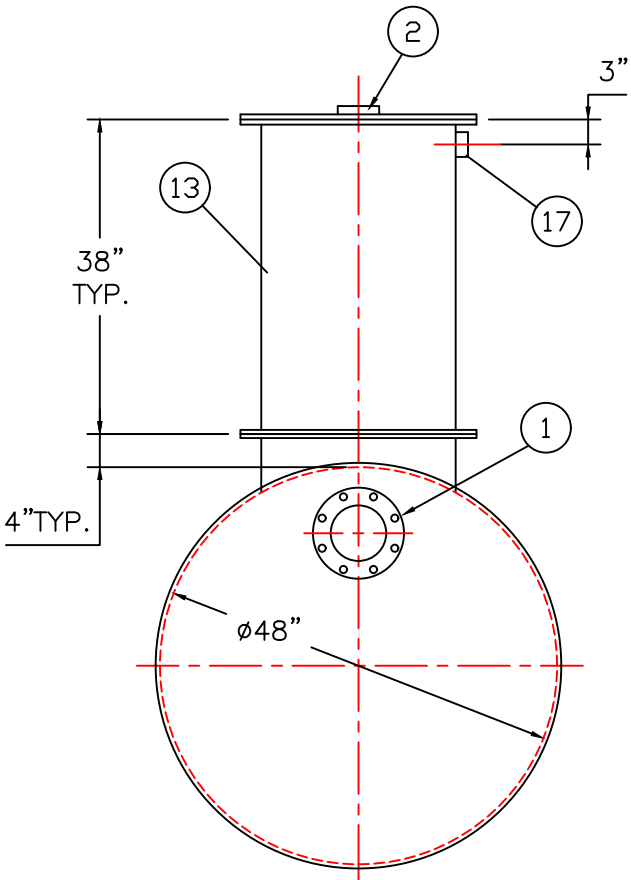
END VIEW
