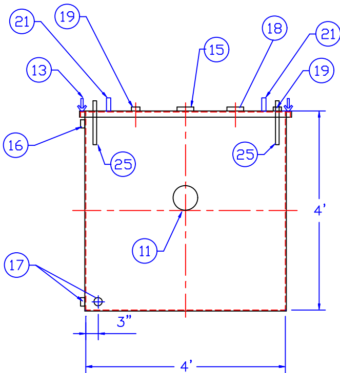
END VIEW
