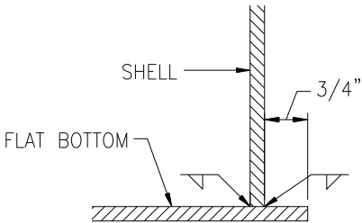
BOTTOM JOINT DETAIL
