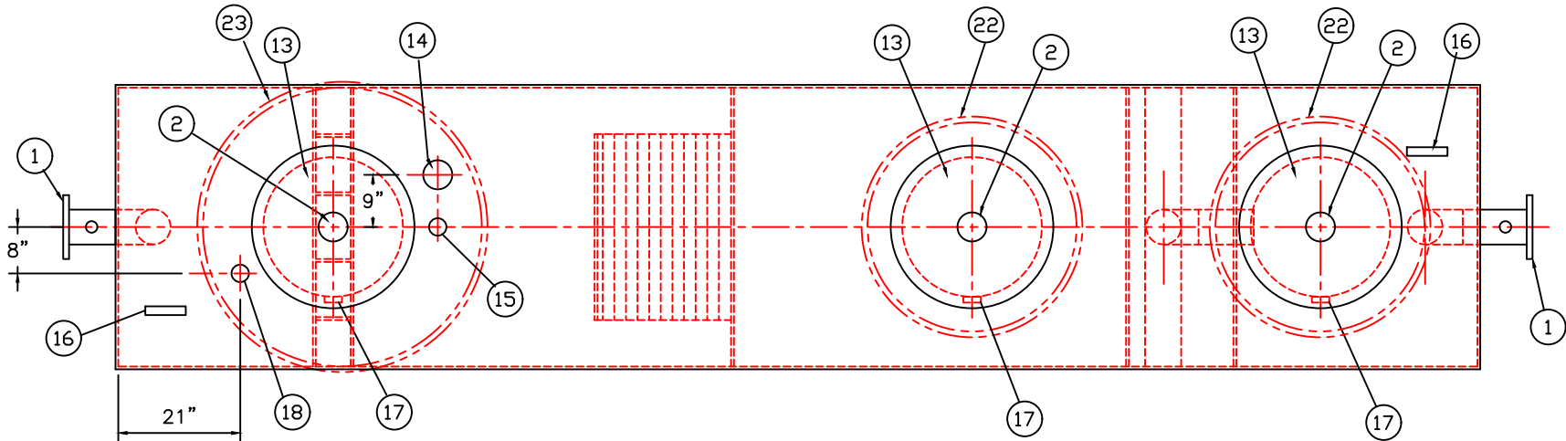
PLAN
