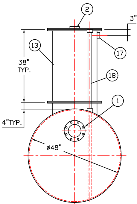
END VIEW
