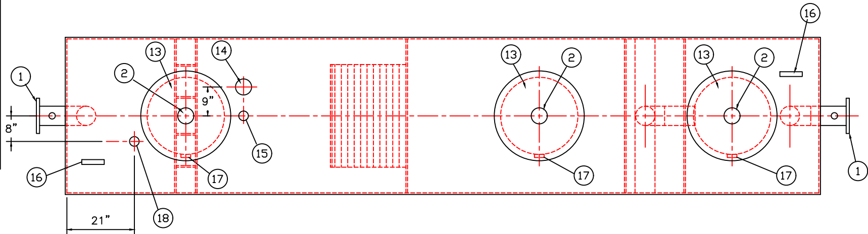
PLAN
