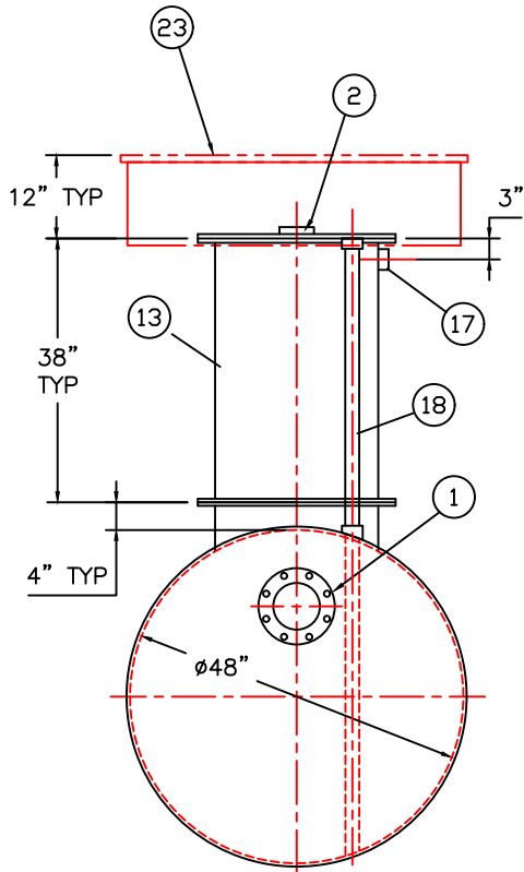
END VIEW
