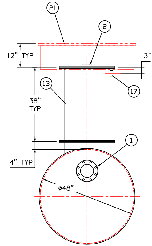
END VIEW
