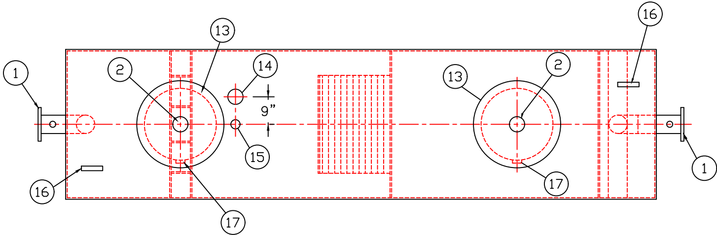
PLAN
