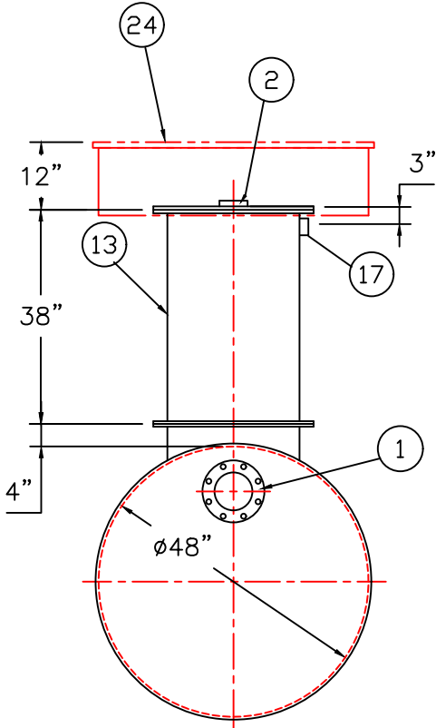
END VIEW
