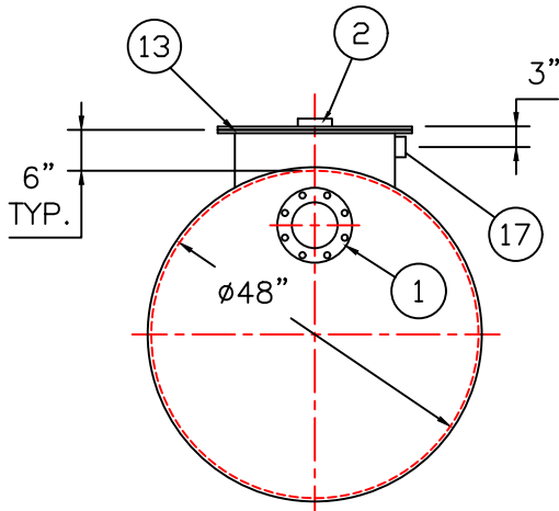
END VIEW
