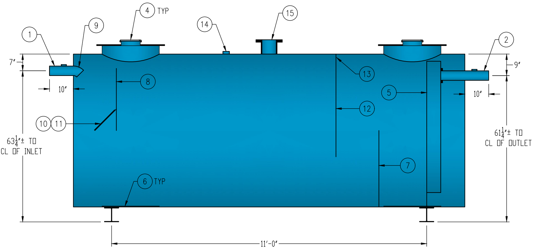
SECTION VIEW
