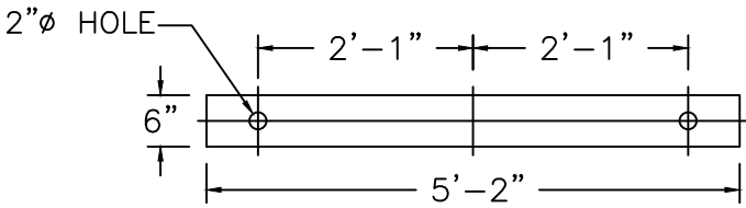
COMMUNICATION BOX DETAIL
