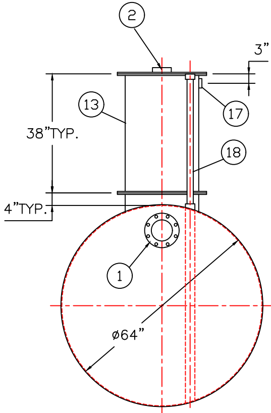
END VIEW
