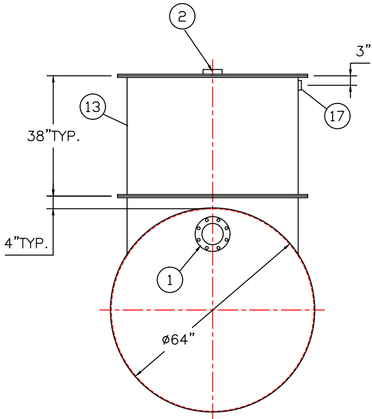
END VIEW
