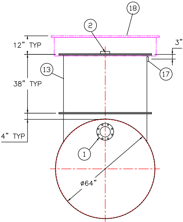
END VIEW
