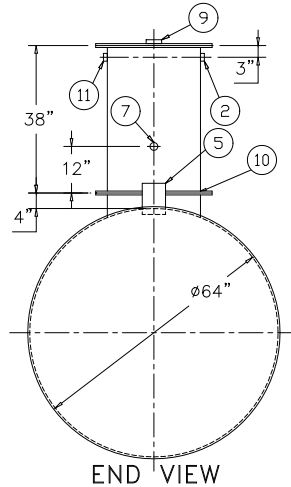
END VIEW
