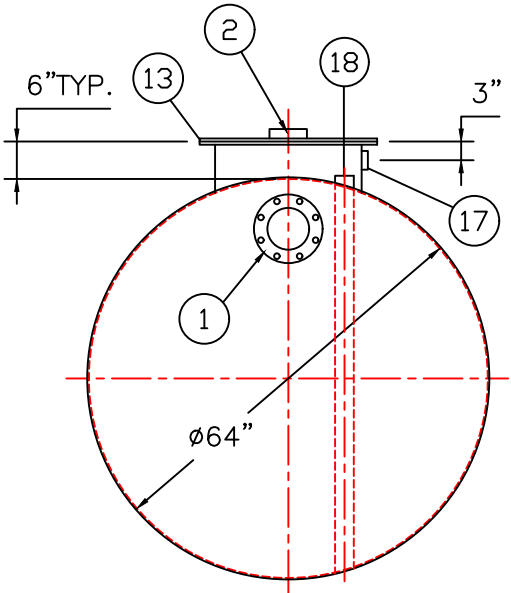
END VIEW
