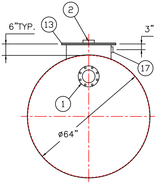
END VIEW
