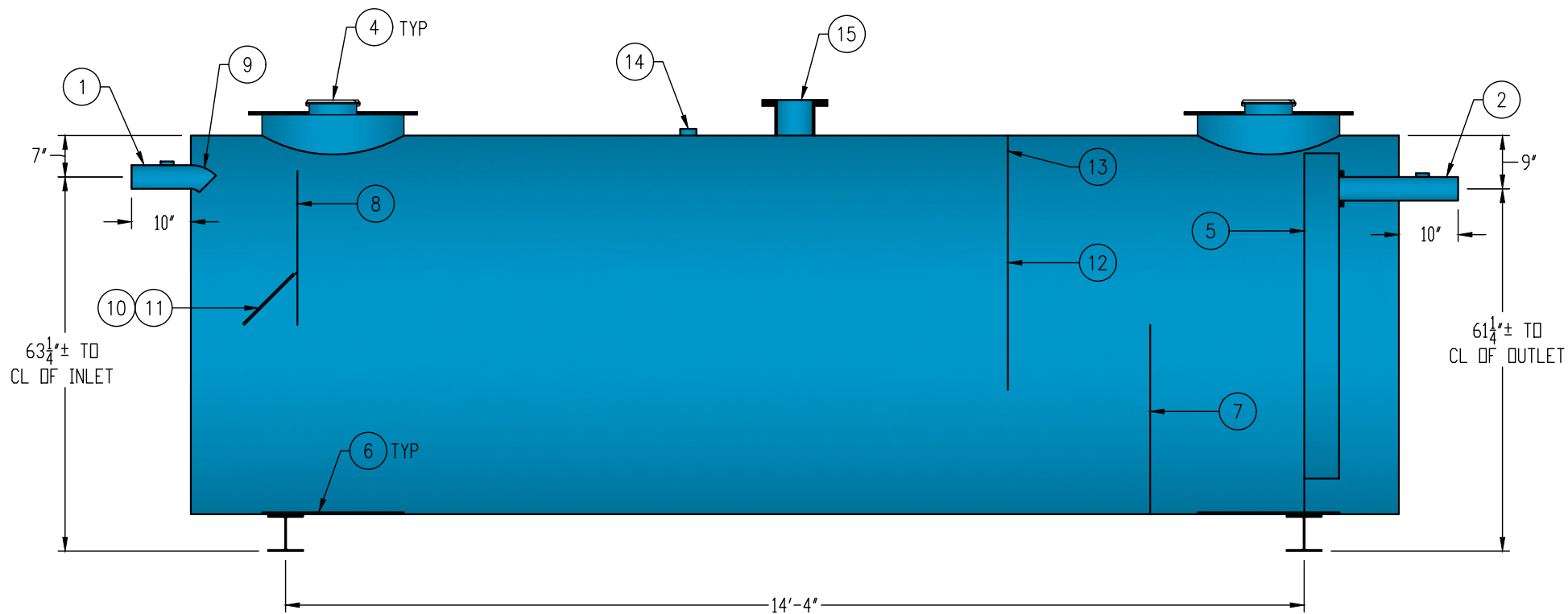
SECTION VIEW
