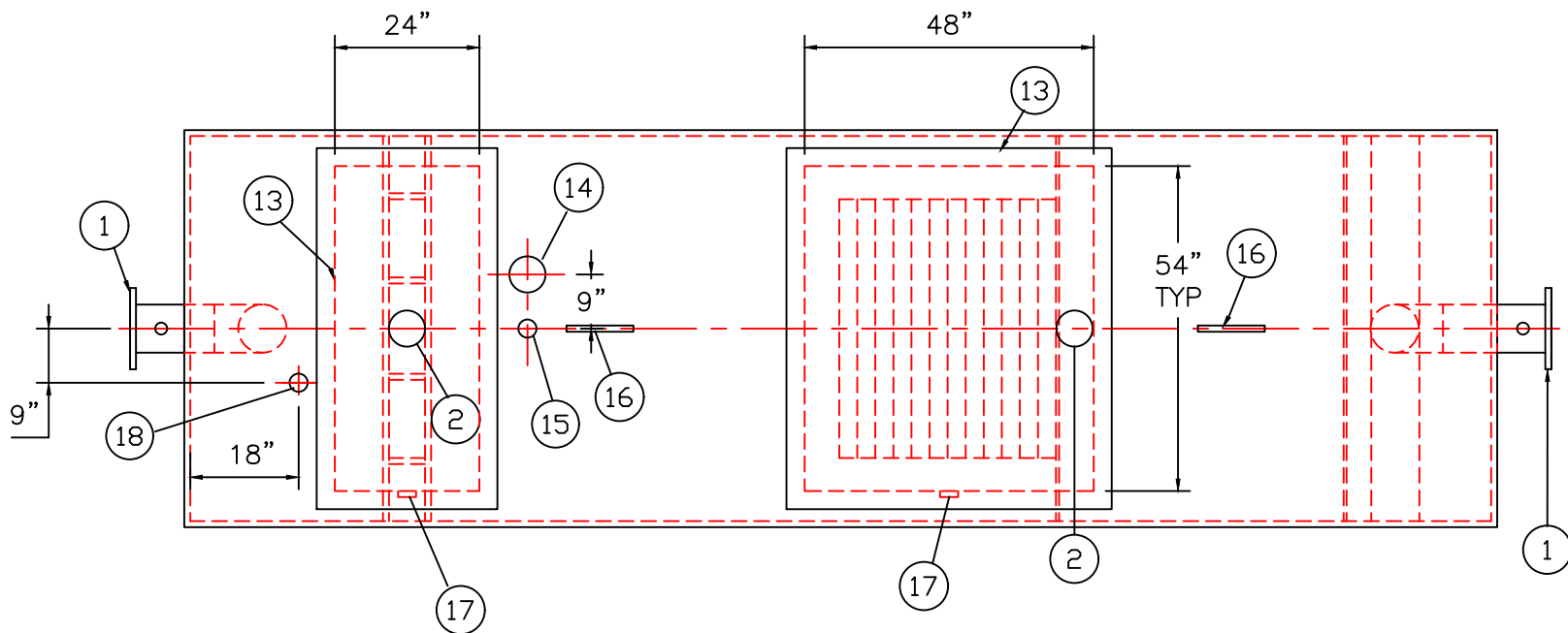
PLAN
