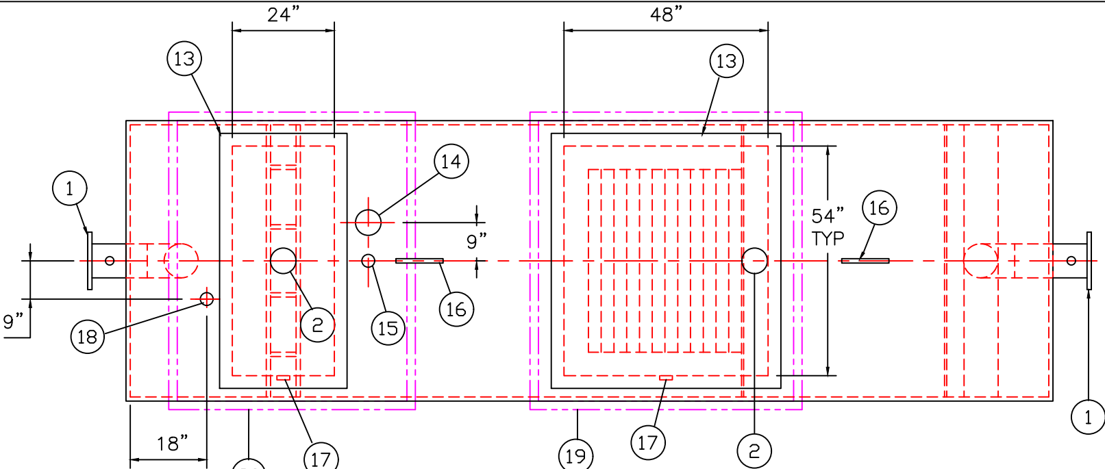
PLAN
