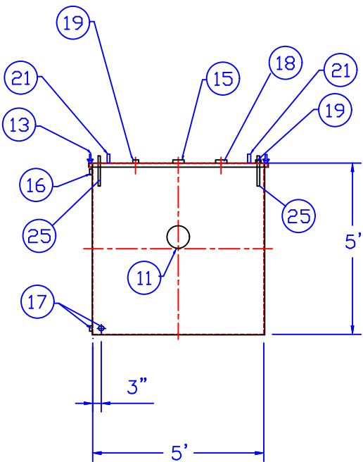
END VIEW
