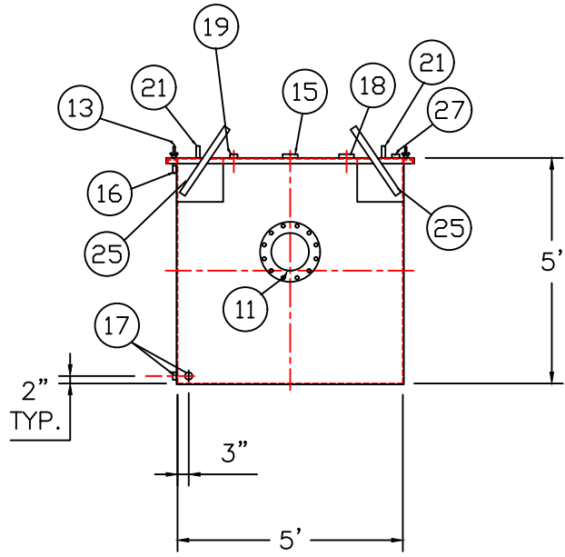
END VIEW
