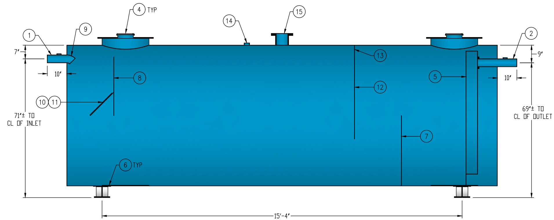
SECTION VIEW
