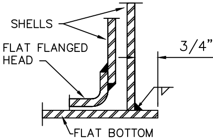
BOTTOM JOINT DETAIL
