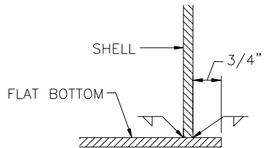
BOTTOM JOINT DETAIL
