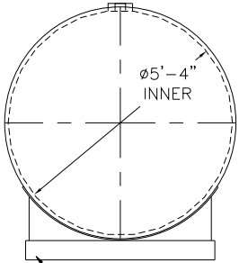
(2) 5'-4"Ø X 6" HIGH SADDLES SHIP LOOSE
