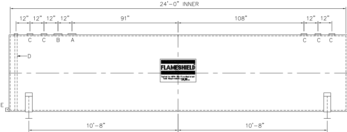
(2) 5'-4"Ø X 6" HIGH SADDLES SHIP LOOSE
