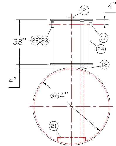
END VIEW
