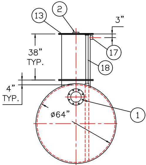
END VIEW
