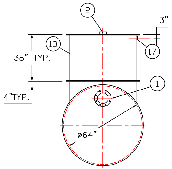
END VIEW
