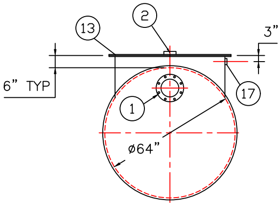
END VIEW
