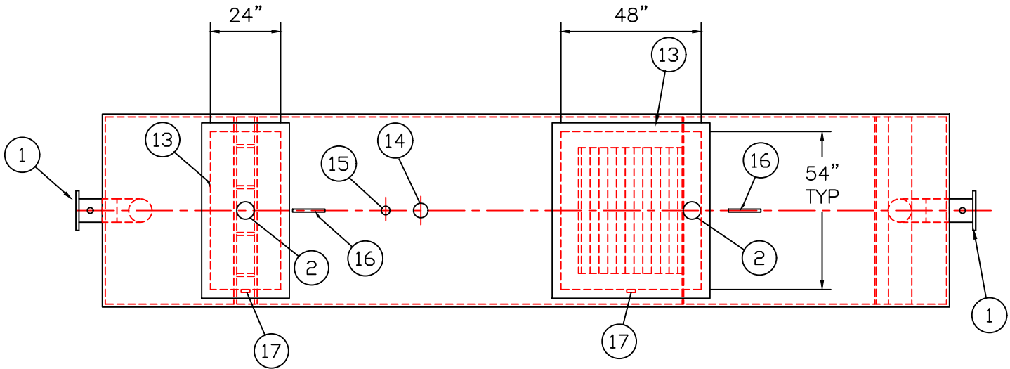
PLAN
