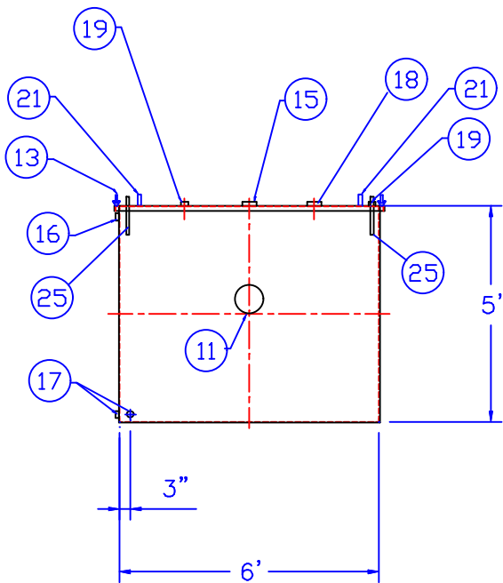
END VIEW
