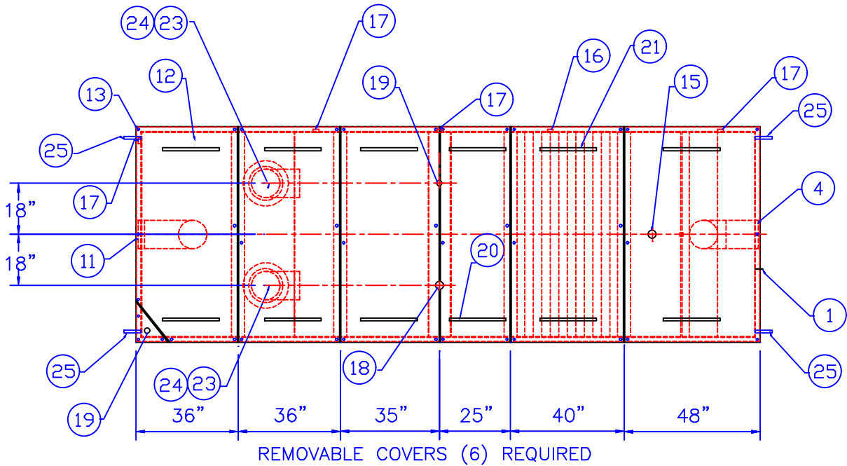
PLAN VIEW
