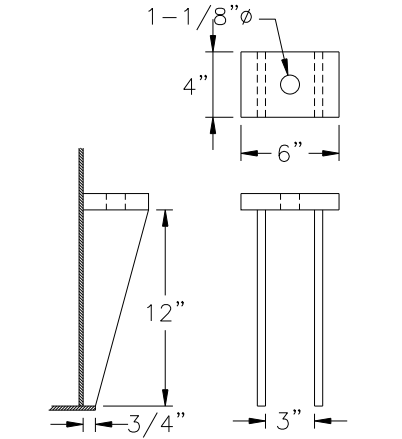
ANCHOR CHAIR DETAIL
