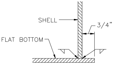
BOTTOM JOINT DETAIL
