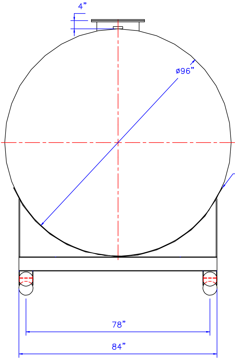
END VIEW
