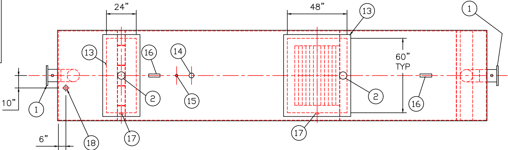
PLAN
