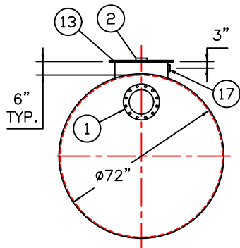
END VIEW
