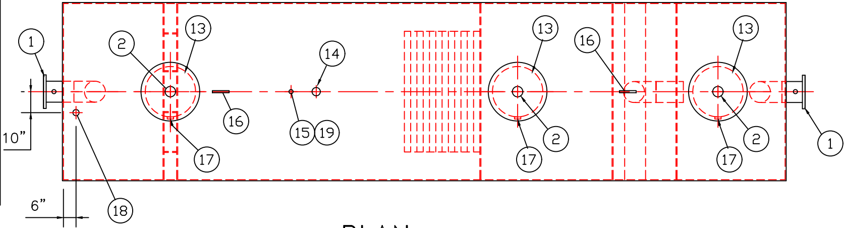
PLAN
