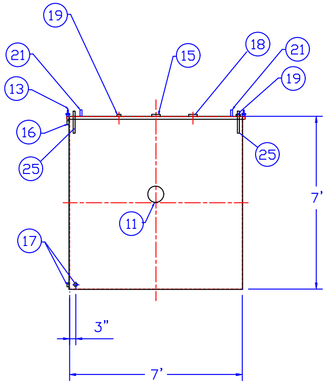
END VIEW
